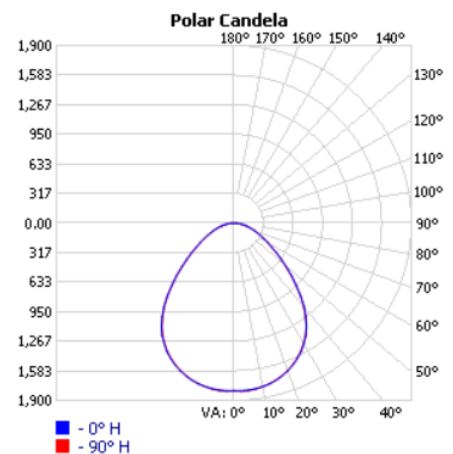
Same luminaire with WhiteOptics glare control (DLC 5.1 Premium UGR)
