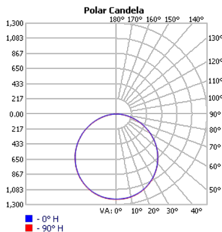
Luminaire with standard diffuser (light in high angles)
