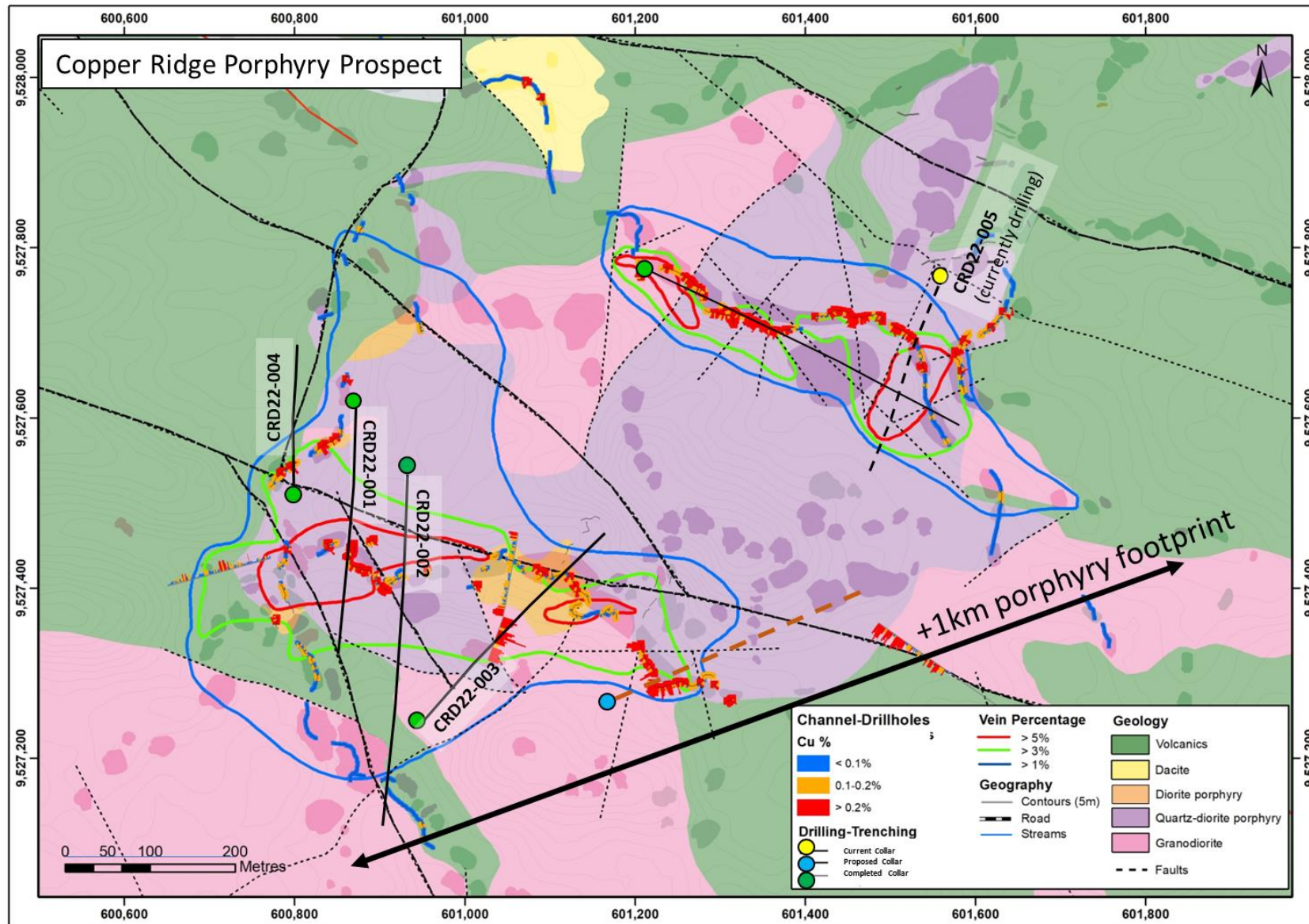
Figure 3: Plan for Copper Ridge prospect, displaying Titan's Drilling, and the relationship between vein abundance and copper anomalies
