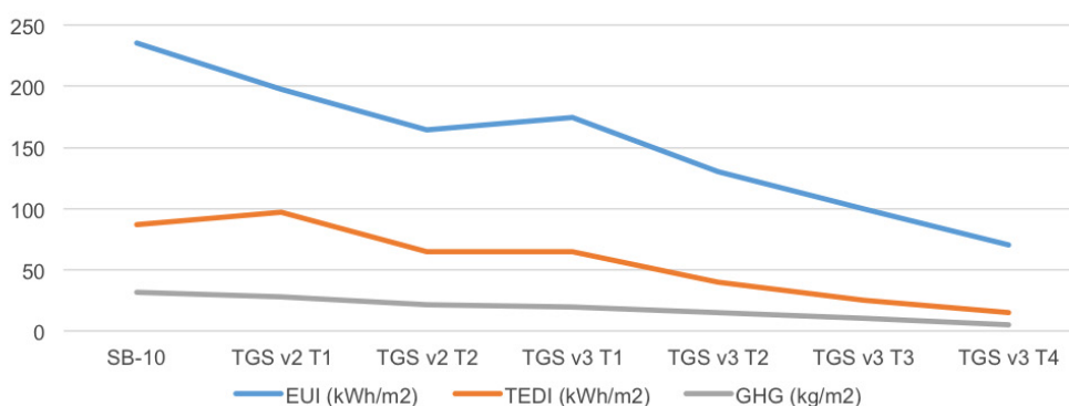
Figure 11: Target progression to near-zero emissions for Low-Rise MURB
